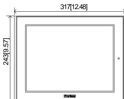
Front View (FP2600-T11)
